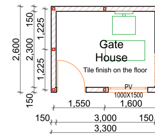
PROPOSED GATE HOUSE
